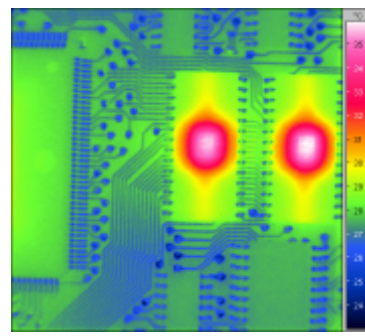
Real-time check of electronic components of a PCB with fast changes of electrical load
