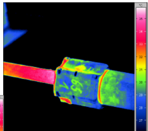
Thermal analysis of the behaviour of a cardan drive with mechanical load
