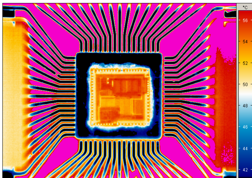
Micro electronic circuit (with macro lens) – View with several colour palettes
