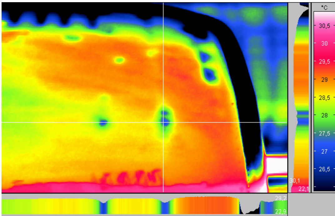
Water inside of the turbine (measurement 45min after landing)
