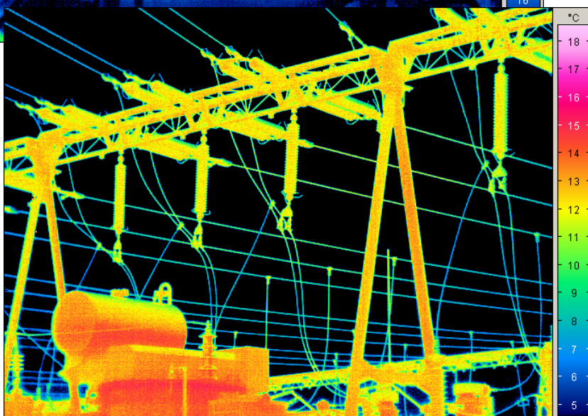
Inspection of isolators and connections in a transformer station
