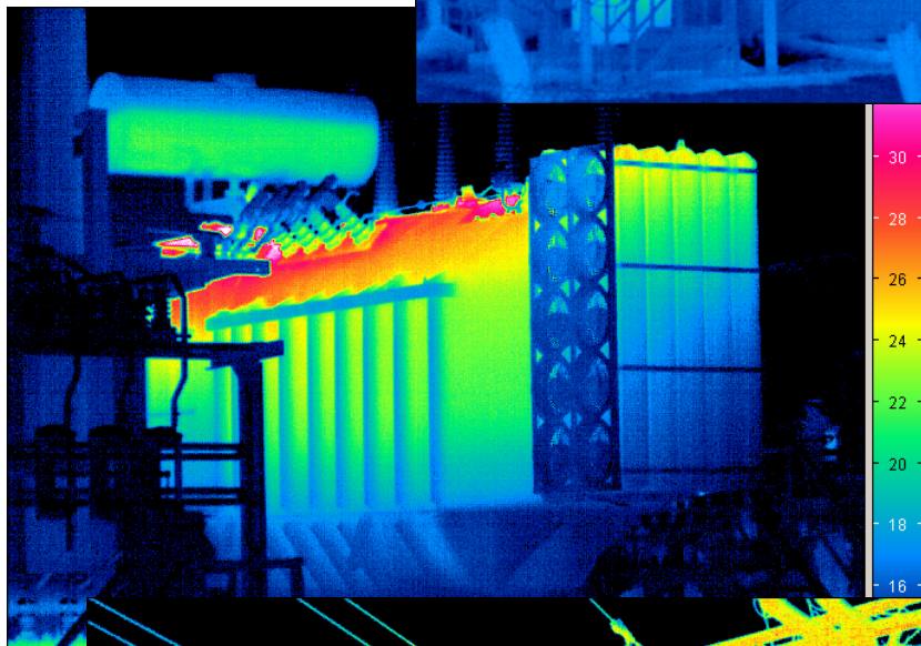
Thermal image with standard and telephoto lens from same distance
