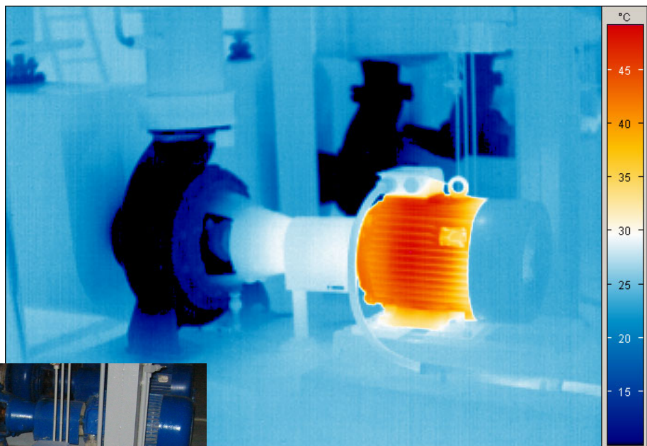
Thermography of a pump aggregate with visual image of the same camera
