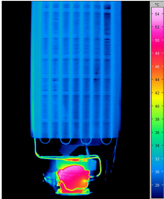
Thermal inspection on different compressors
