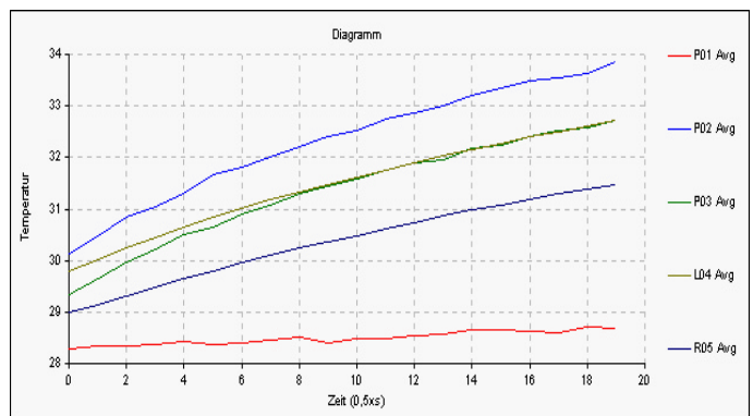
Temperature-time process on the basis the defined measuring points (standard objective and macro adapter)
